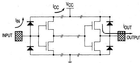
Figure 4-12. Noise Effects
