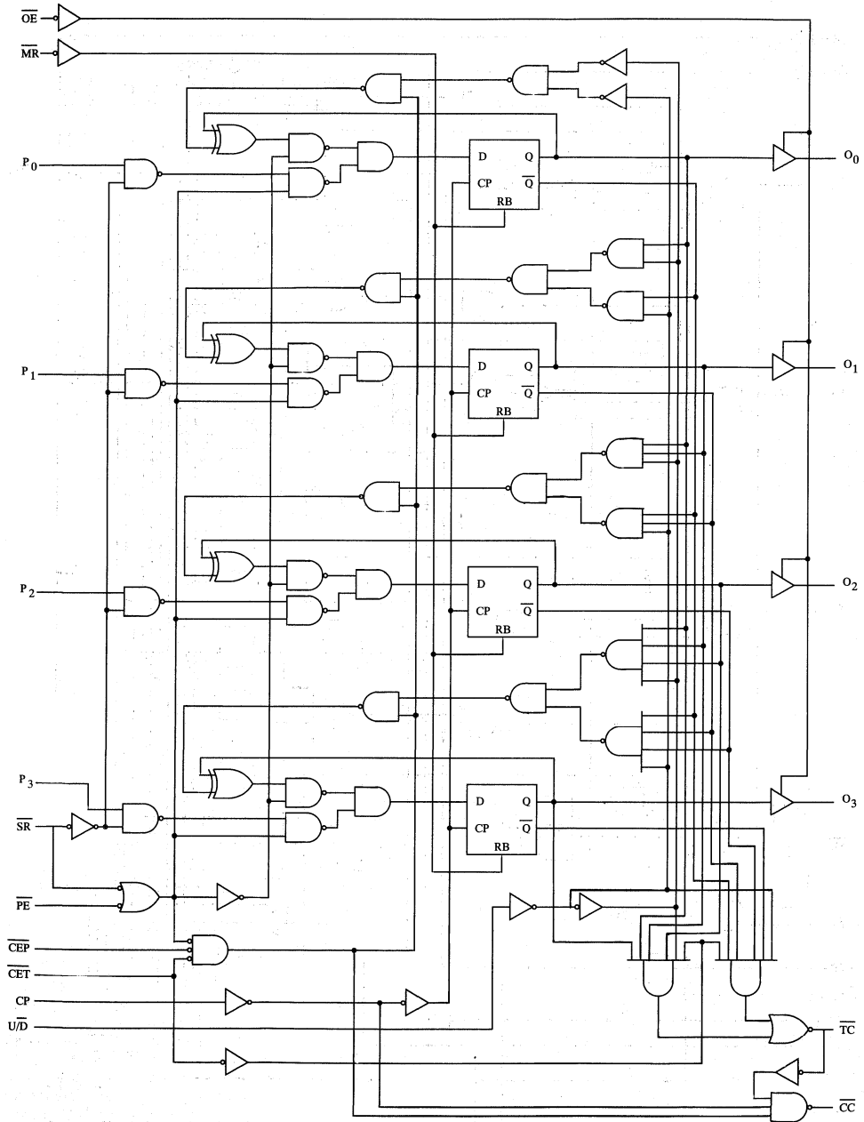
Logic Diagram (AC569)
