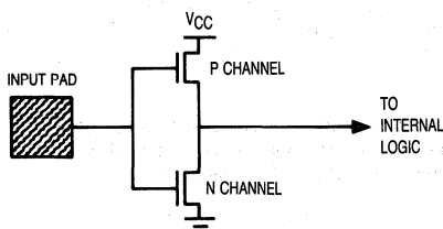
Figure 4-20. CMOS Input Structure
