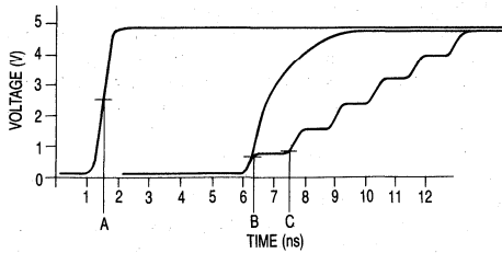
Figure 4-28. Measurement Stepout
