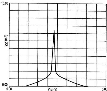
Figure 4-22. I_{CC} versus I_{IN}
