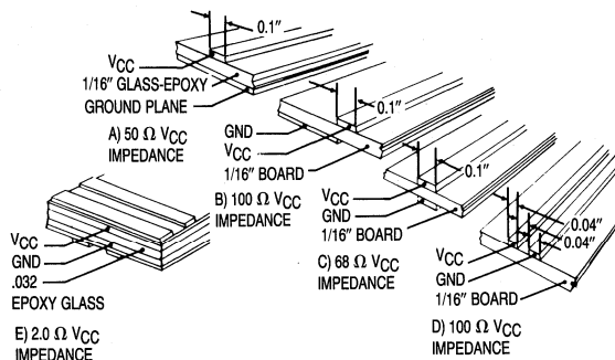
Figure 4-17. Power Distribution Impedances
