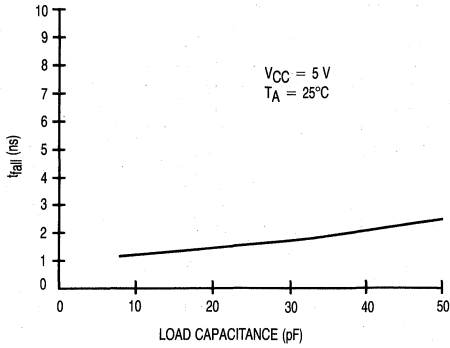
Figure 2-15. t_{fall} versus Capacitance
