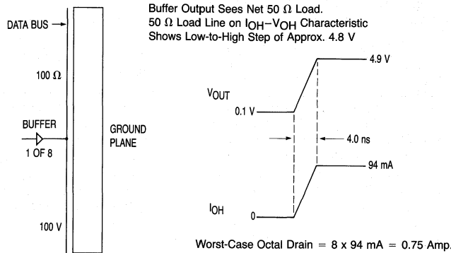
Figure 4-18. Octal Buffer Driving a 100 Ohm Bus
