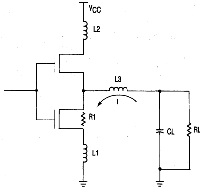
Figure 4-16b. Output Voltage
