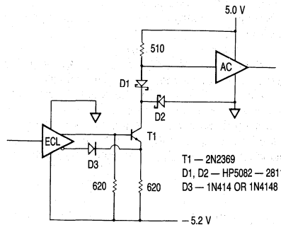
Figure 4-8c. Differential Output ECL-to-'AC Circuit
