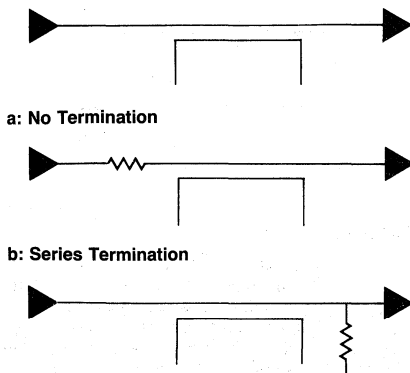
Figure 4-10. Termination Schemes
