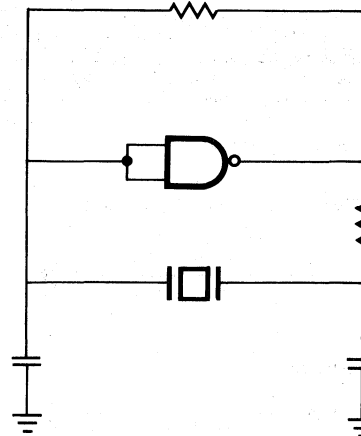
Figure 4-9. Crystal Oscillator Circuit Implemented with FACT 'AC00
