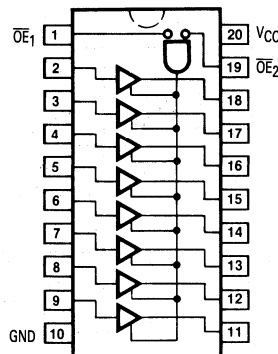
MC74AC541/74ACT541
