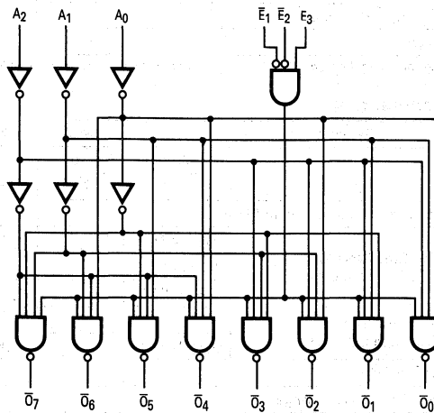
LOGIC DIAGRAM
