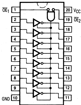
MC74AC540/74ACT540
