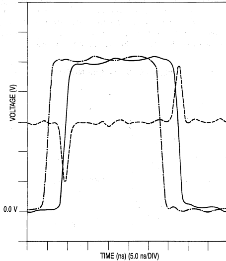
Figure 4-13a. Forward Crosstalk on PCB Traces
