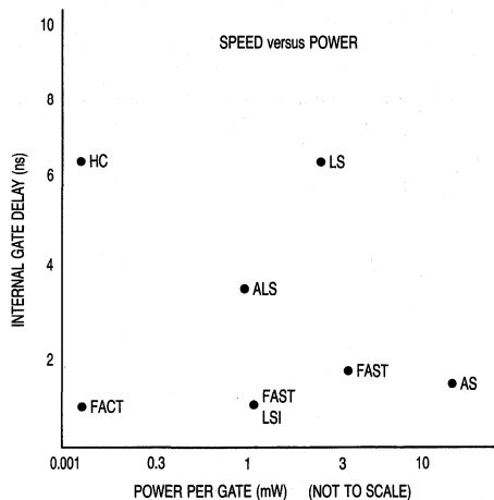
Figure 2-7. Internal Gate Delays
