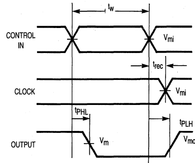
Figure 3-6. Propagation Delay, Pulse Width and t_{rec} Waveforms
